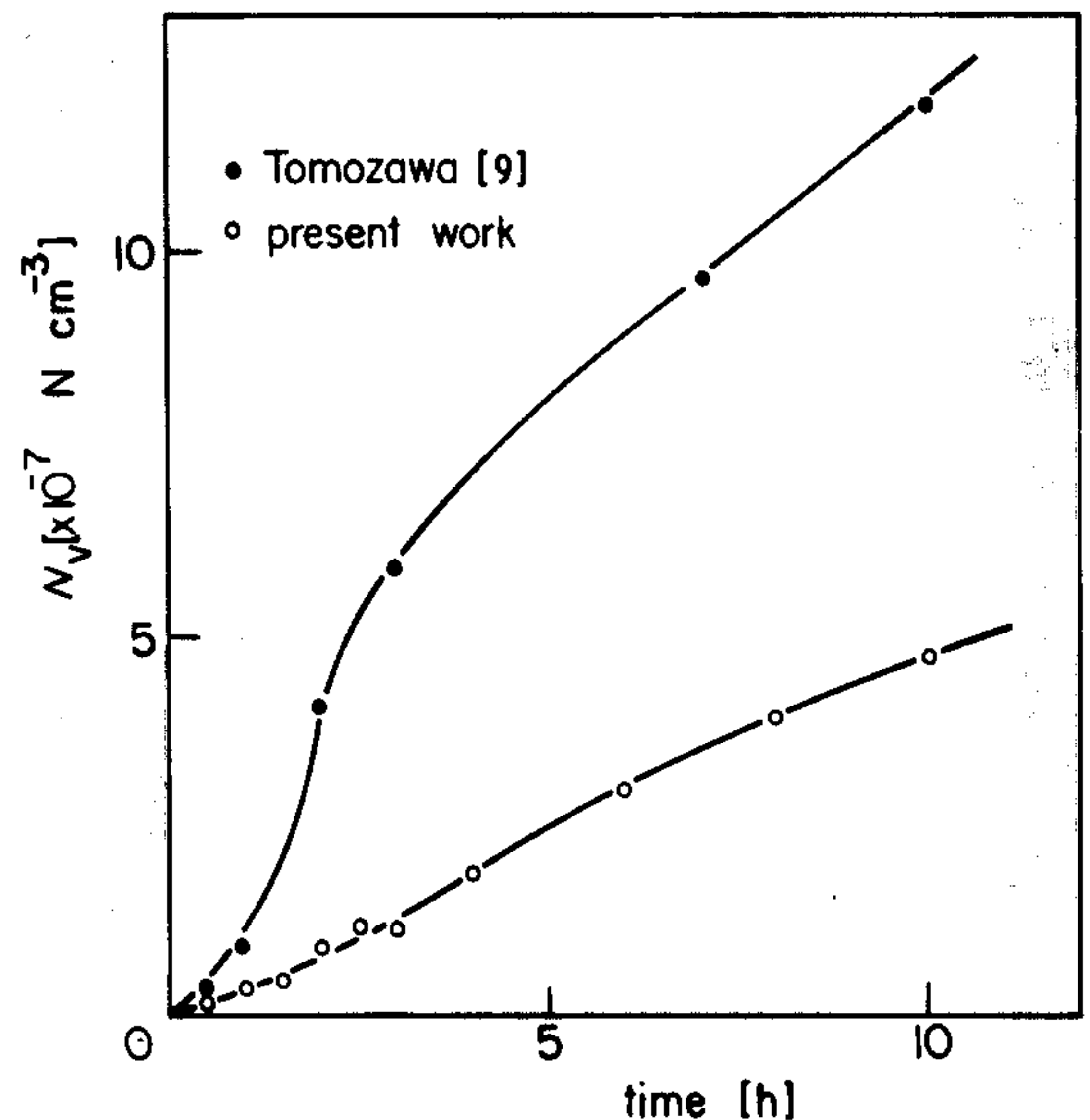
Figure 9 Crystal nucleation curves of nominally 31.0 mol% \text{Li}_2\text{O} glasses nucleated at 475^\circ\text{C} , from Tomozawa [9] and present work.
