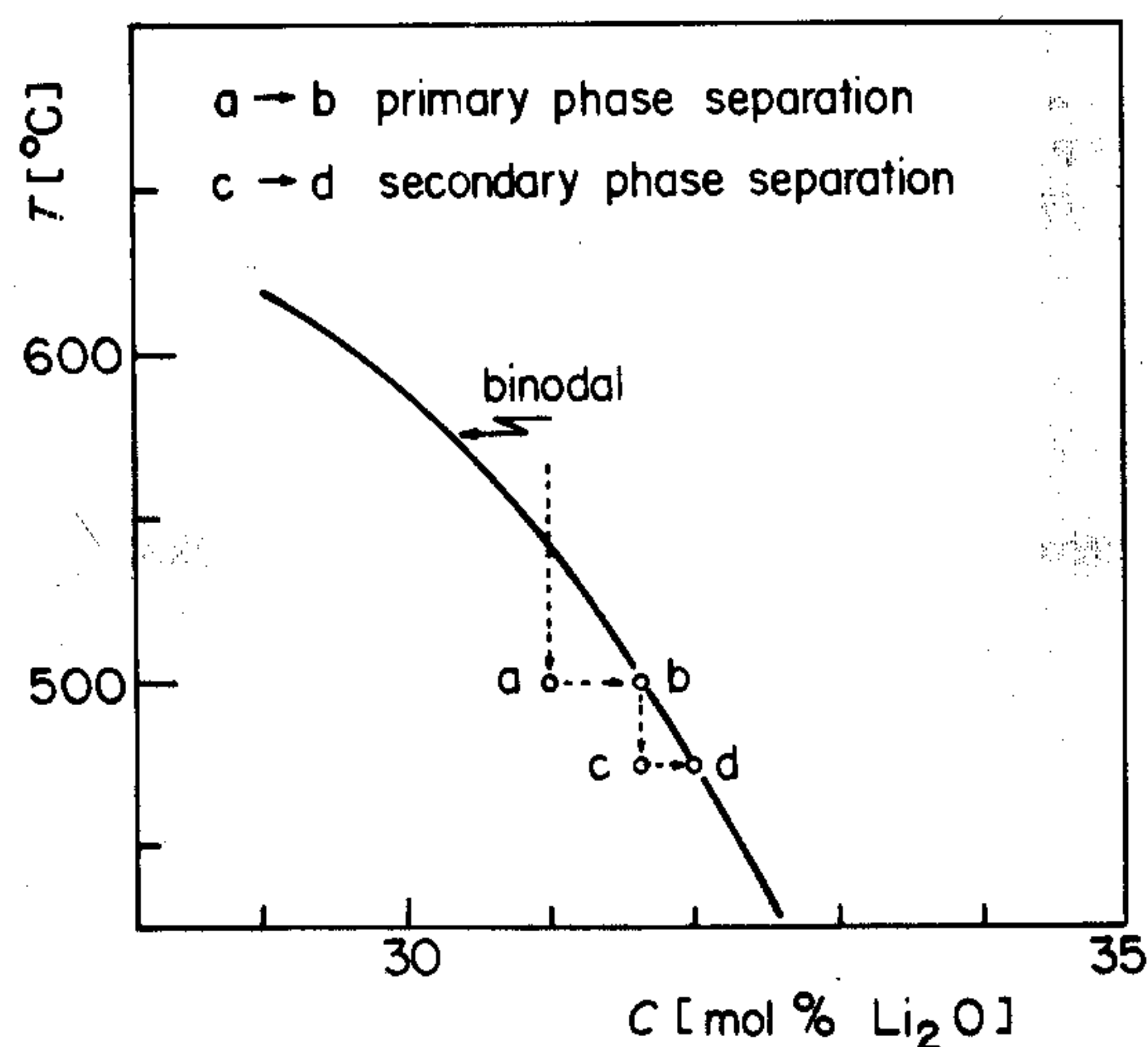
Figure 12 Schematic composition path of the matrix of samples heat treated at 500°C first and at 475°C later.
