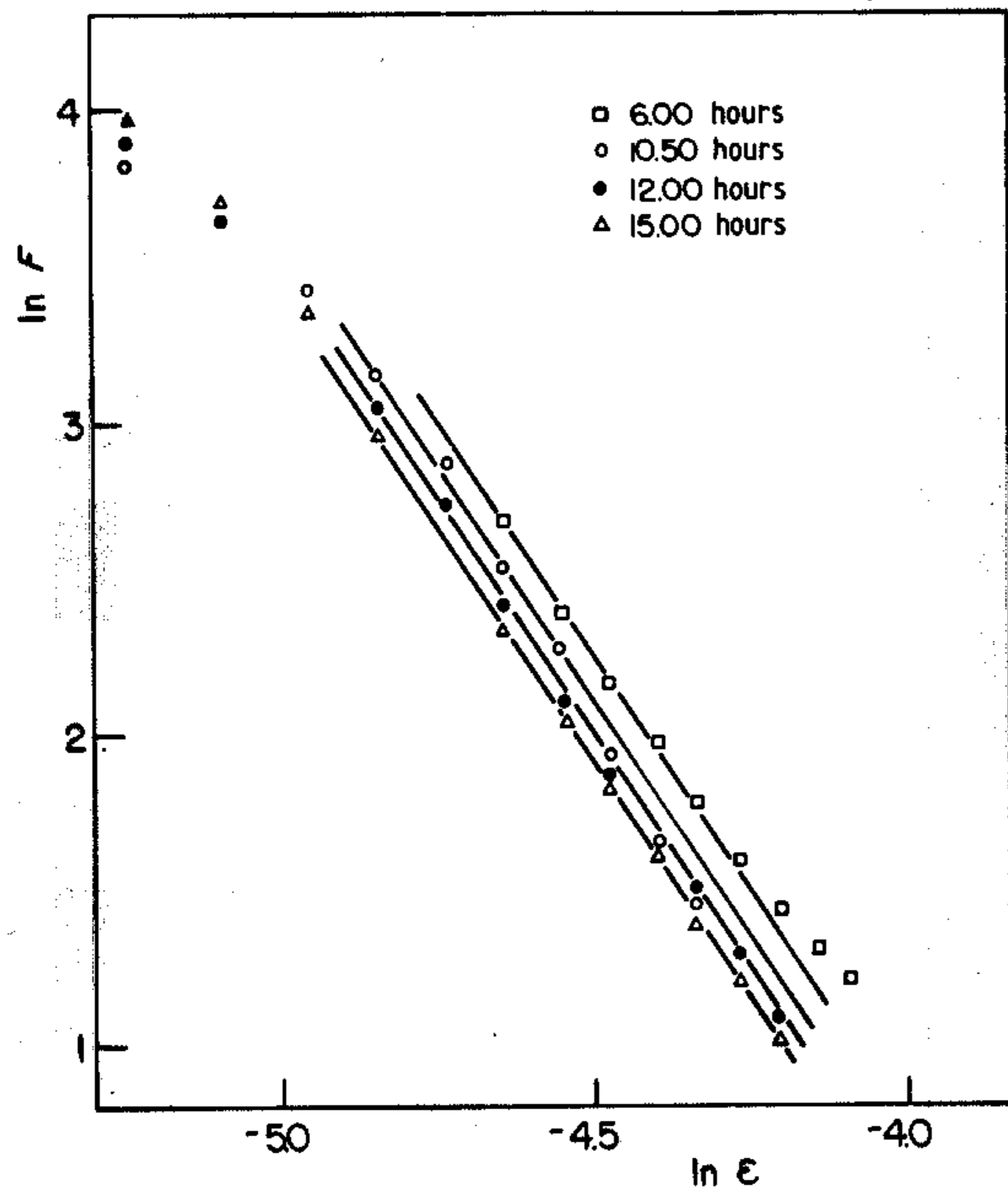
Figure 4 Porod plots of 31.0 mol% \text{Li}_2\text{O} glasses heat treated at 475^\circ\text{C} .
