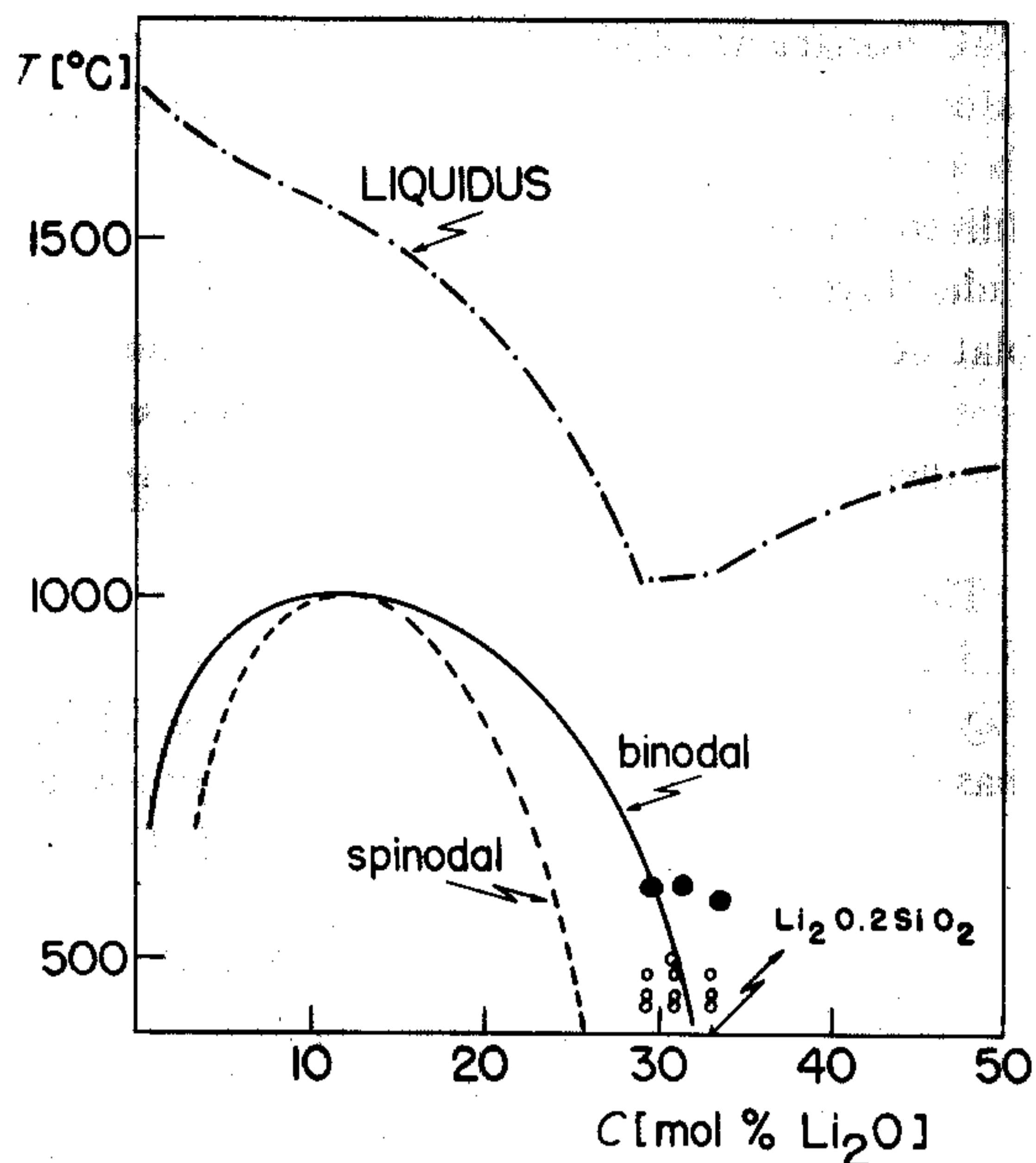
Figure 1 Miscibility gap in the \text{Li}_2\text{O}-\text{SiO}_2 system according to the literature [9] showing the location of the nucleation (○) and growth (●) heat treatments employed (nominal glass compositions).
