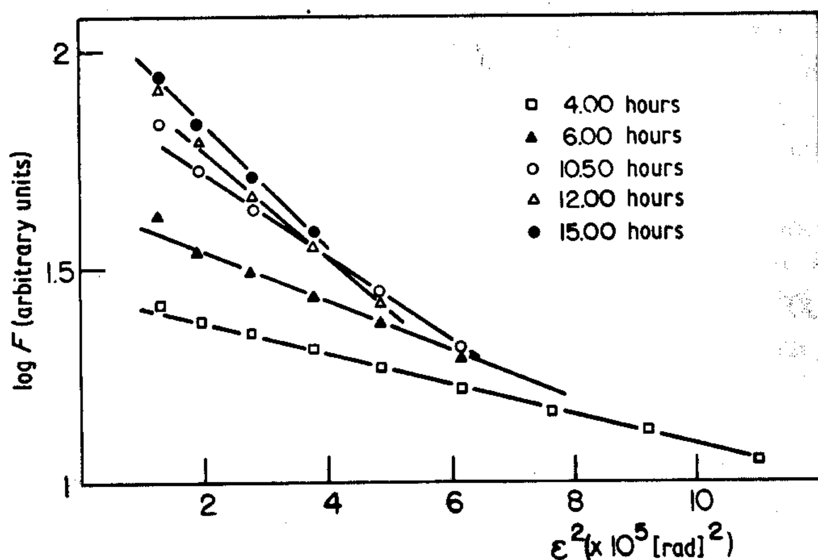
Figure 3 Guinier plots of 31.0 mol% \text{Li}_2\text{O} glass samples heat treated at 475^\circ\text{C} .
